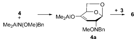
Scheme 3. One-pot double addition.
