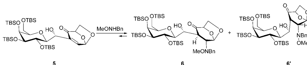
Scheme 2. Reversible addition of methoxybenzylamine to enone 5 .
