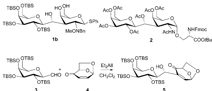
Scheme 1. Synthesis of C(1→3)-disaccharide precursors.
