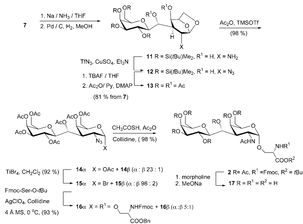
Scheme 5. Synthesis of C-linked disaccharide \alpha -O-conjugated to L-serine.
