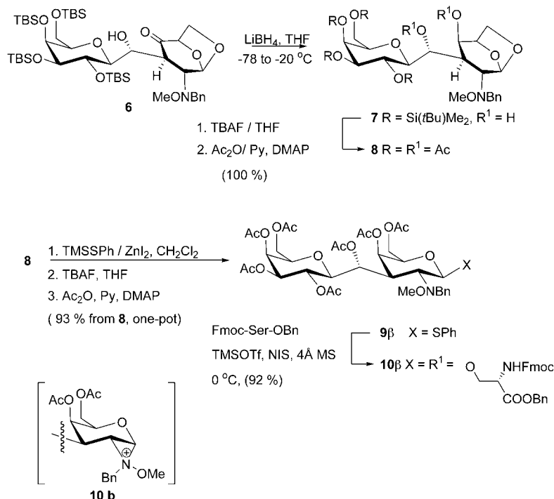
Scheme 4. \beta -O-Galactosidation: participation by the 2-methoxy (benzyl)-amino group.
